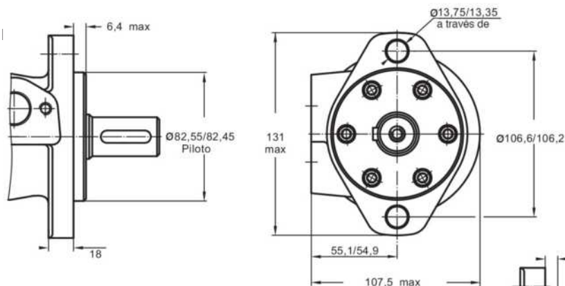
F Brida Magneto
