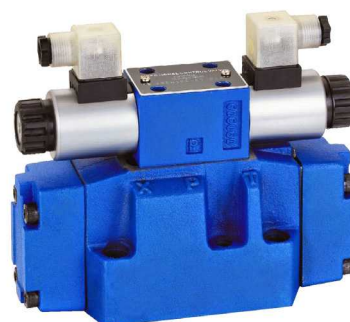
4 WEH 16..-5X/..6E..N..S..K4..
